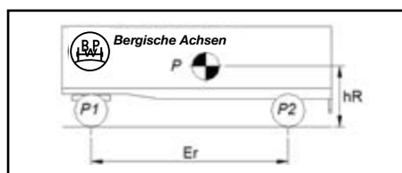
Two Axle Drawbar Trailer
