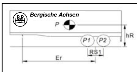
Tandem Axle Semi-Trailer
