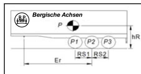
Tri-Axle Semi-Trailer
