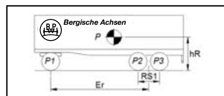
Three Axle Drawbar Trailer
